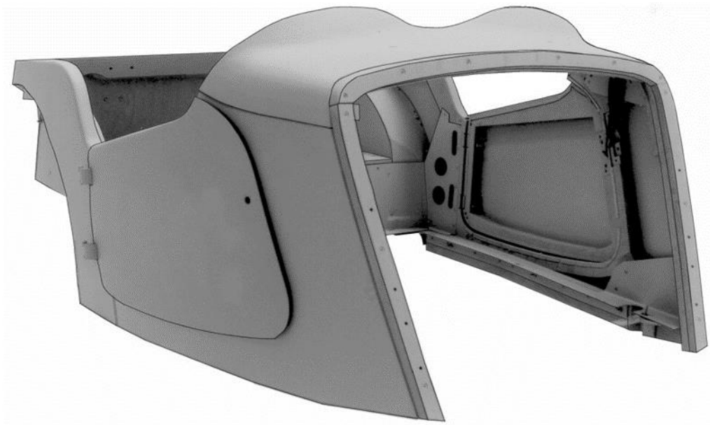
Fully Assembled Steel Panelled Body. TA-TF With Scuttle Top, Hinges & Doors Hung
