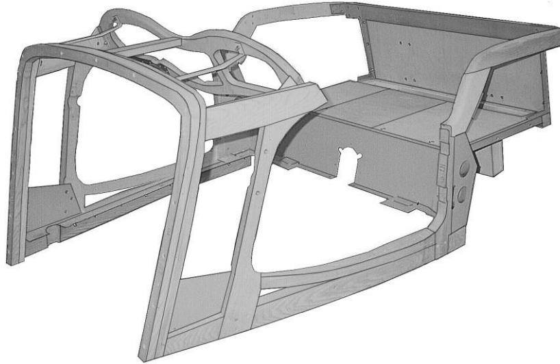
Fully Assembled Ash Frame Skeleton. TA-TF (Also available in kit form)
